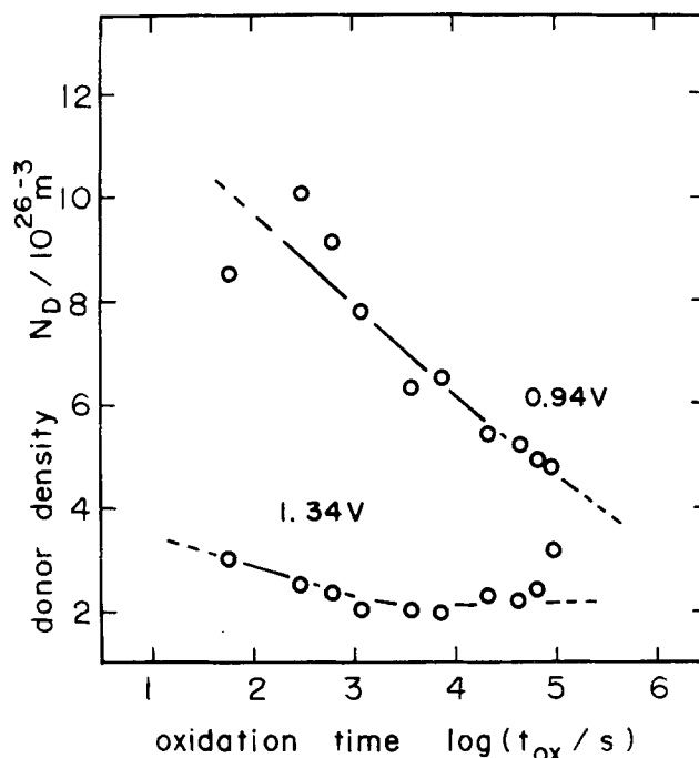
Fig. 8. Value of N_D vs. oxidation time t_{ox} for the passive film formed on iron at 0.94 and 1.34V in pH 6.5 borate solution. The impedance was measured at a fixed frequency of 1.00 Hz.
